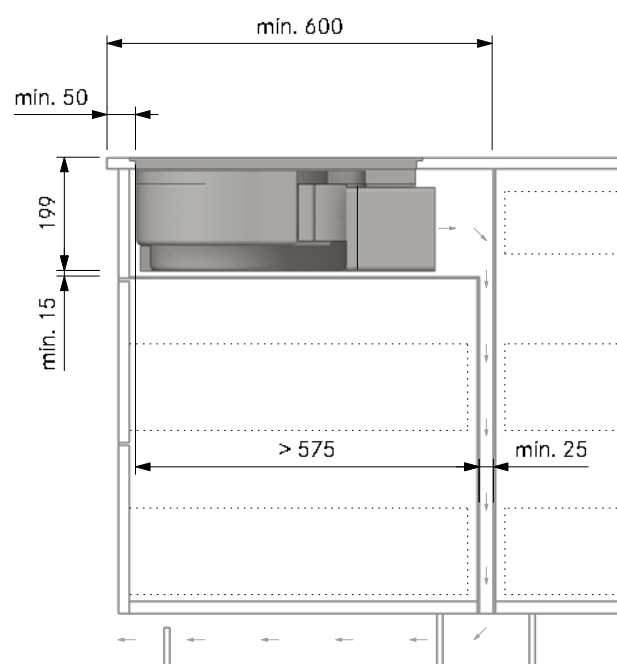
Installation cut-out PURSU with reversible false floor (kitchen island):
