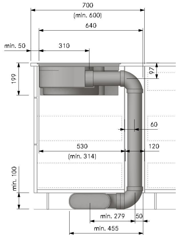
Installation cut-out PURSA (kitchen island):
